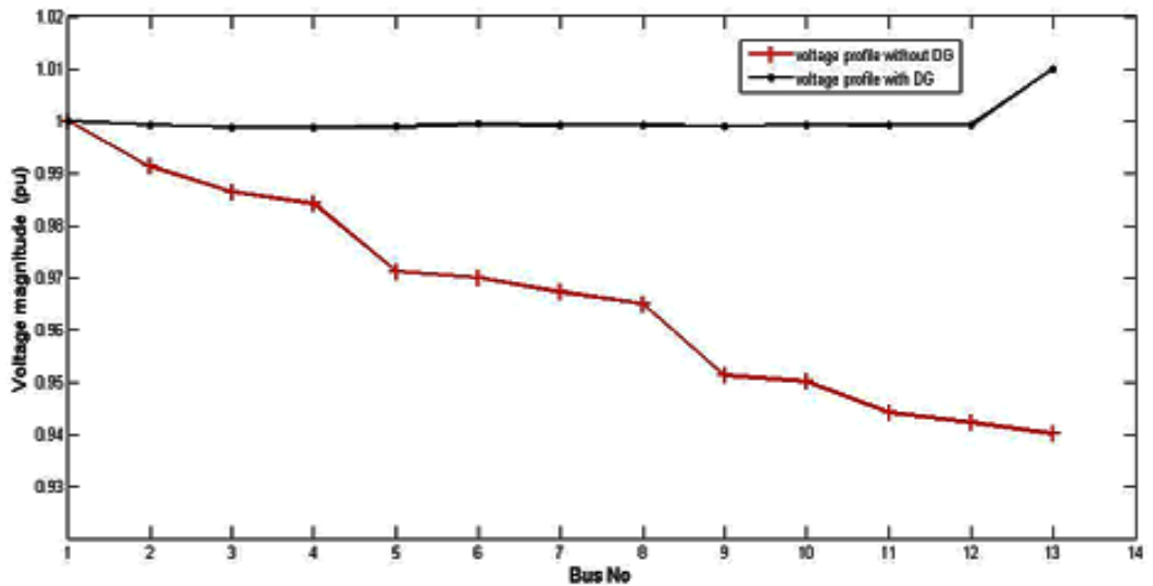
Figure 9. Voltage magnitudes with and without DG for IEEE-13 bus
