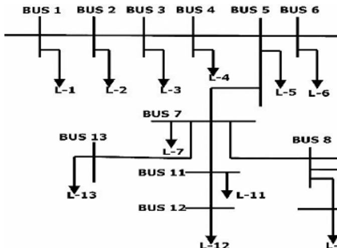
Figure 7. IEEE-13 Bus standard test system
