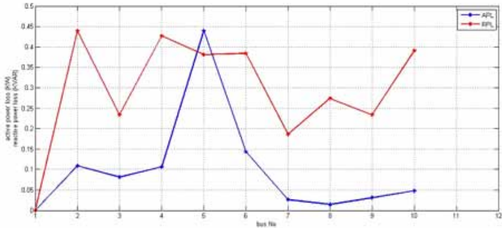
Figure 4. Real and reactive power of IEEE-10 Bus system
