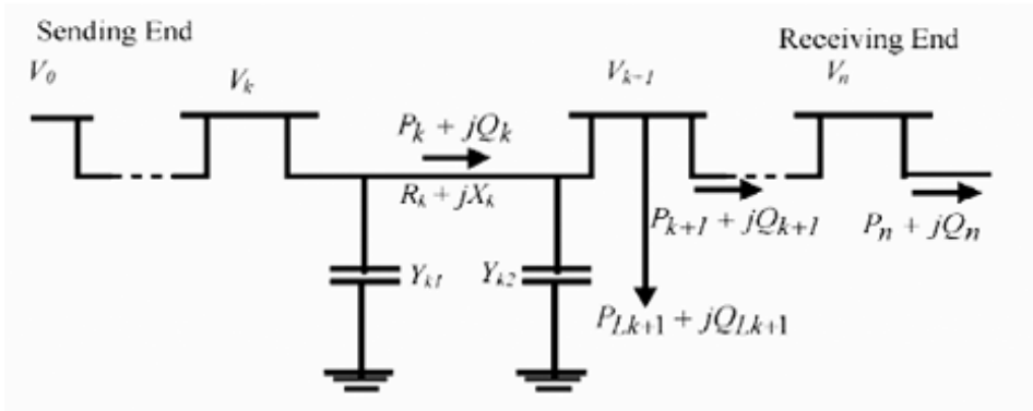
Figure 1. Single-line diagram of RDS
