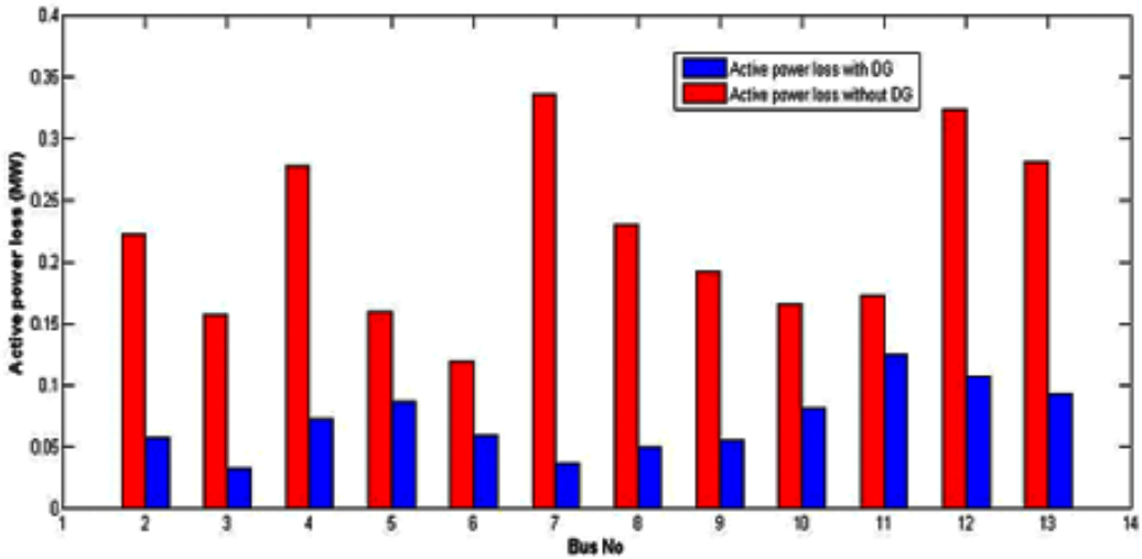
Figure 10. Active power loss reductions for IEEE-13 Bus system
