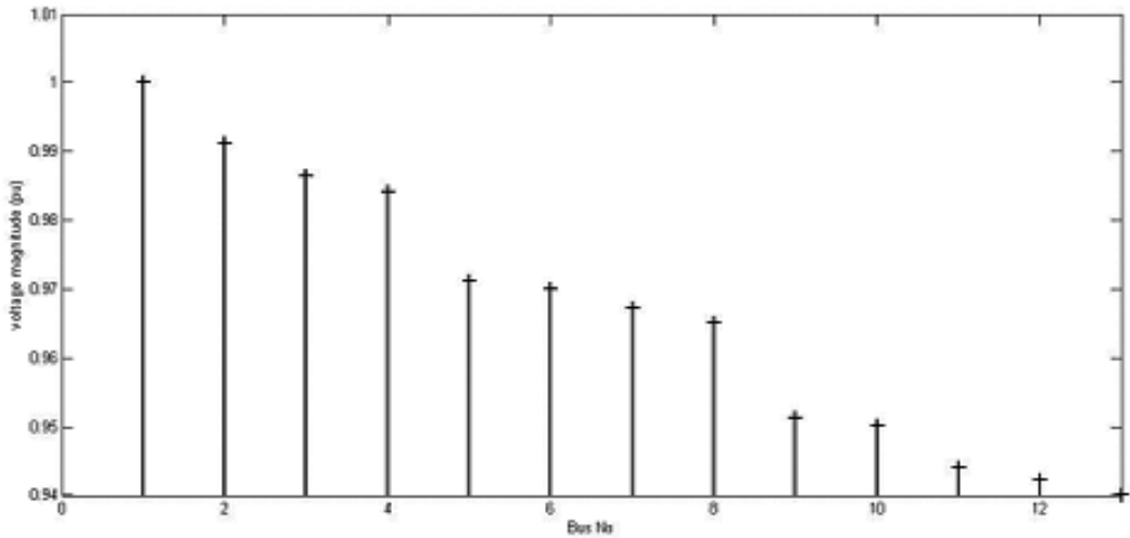
Figure 8. Voltage profile for IEEE-13 Bus system
