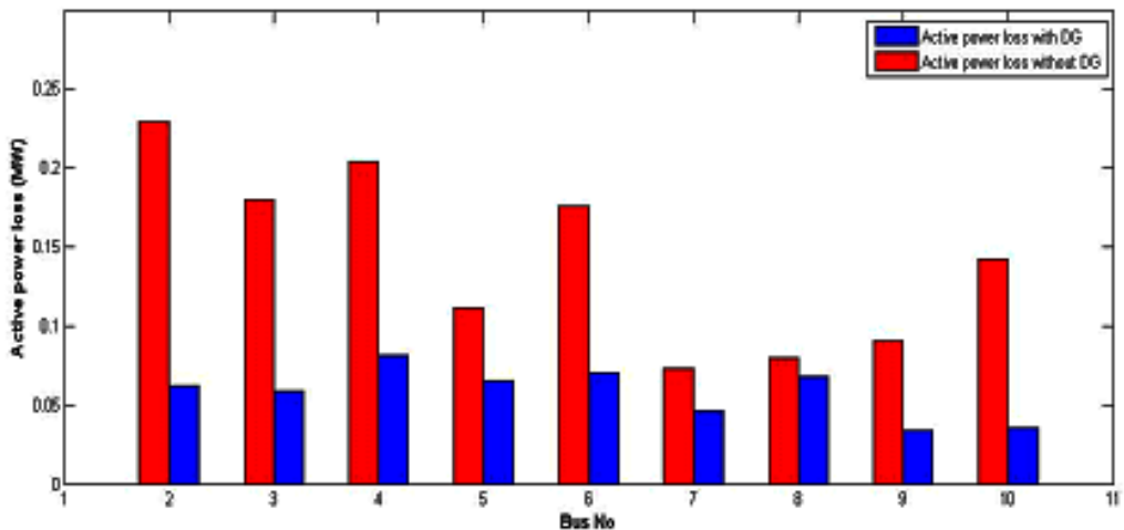
Figure 6. Active power loss reductions for IEEE-10 Bus
