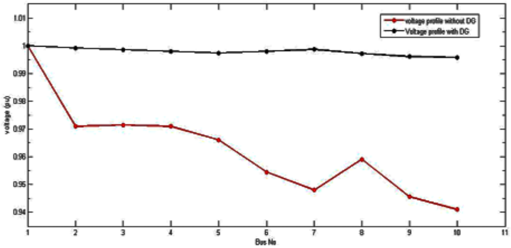
Figure 5. Voltage profile improvement for the IEEE-10 Bus system
