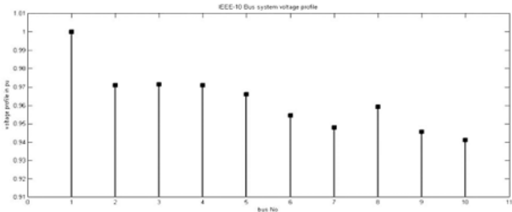
Figure 3. Voltage profile for IEEE-10 Bus system
