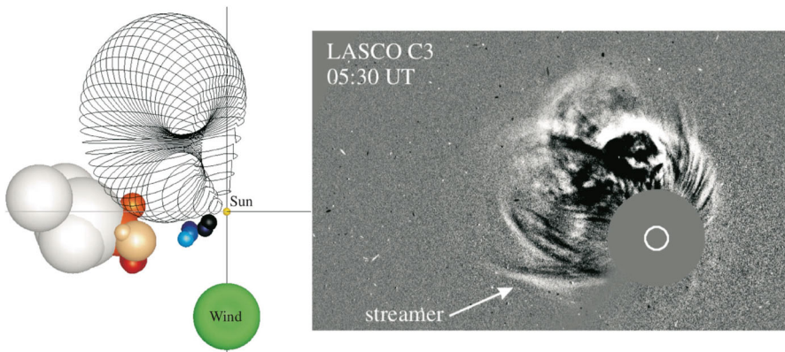
Fig. 16 Left panel: View of the flux rope and radio sources as seen from Earth. The CME flux rope obtained from GCS 3D reconstruction (black grid croissant) together with the 3D reconstruction of the radio type II burst (dark and light blue spheres) using gonopolarimetric technique. Right panel: SOHO/LASCO C3 difference image showing the CME as seen from Earth, for comparison with the left panel. Image adapted from Magdalenic et al. (2014), copyright by AGU
