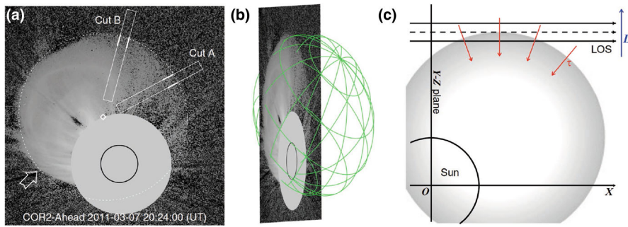
Fig. 14 CME from March 7, 2011: a Excess brightness image from STEREO-A COR2. 3D shock front (green mesh in panel b ) projected on the image plane is shown with the dotted line. The diamond marks the geometric center of the ellipsoid model projected onto the same plane. b Excess brightness in panel a with the 3D shock front (green mesh) modeled with the ellipsoid model described in Kwon and Vourlidas (2017). c Geometric relation among the Sun, shell-like sheath, and line-of-sight. A partial circle around the origin O is the solar disk. A shell-like sheath is represented in gray color. Arrows in black, blue and red are the line-of-sight, the projected shock normal on the image plane, and the actual shock normal in 3D, respectively. Image reproduced with permission from Kwon and Vourlidas (2018), copyright by the authors
