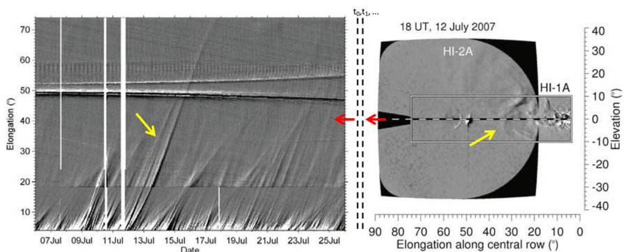
Fig. 17 From running difference STEREO-A HI1+2 image data the central rows are extracted (right) at each time step and rotated by 90 degrees (middle). From this a time-elongation plot (so-called Jmap) is constructed (left). The CME front is marked by a yellow arrow in the direct image as well as in the Jmap. Image adapted from Davies et al. (2009), copyright by AGU
