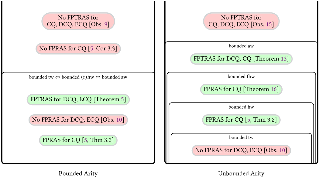
Fig. 1. Overview of our results on approximately counting answers to CQs, to CQs with disequalities (DCQs), and to CQs with disequalities and negations (ECQs). Upper and lower bounds depend on a variety of width measures of the input queries, namely, treewidth (tw), hypertreewidth (hw), fractional hypertreewidth (fhw), and adaptive width (aw). The equivalence of the width parameters in the case of bounded arity is well known; we provide an explicit argument in Observation 34. For completeness, we also compare our results to recent work of Arenas et al. [5]. The lower bounds either rely on the assumption that NP \neq RP or on the rETH. All referenced theorems and observations are stated in Section 1.2. Note that, while our results complete the picture of the complexity of CQ, DCQ, and ECQ in the bounded arity case, two questions remain open for the unbounded arity case: Assuming the adaptive width is bounded, does ECQ have an FPTRAS, and does CQ have an FPRAS?
