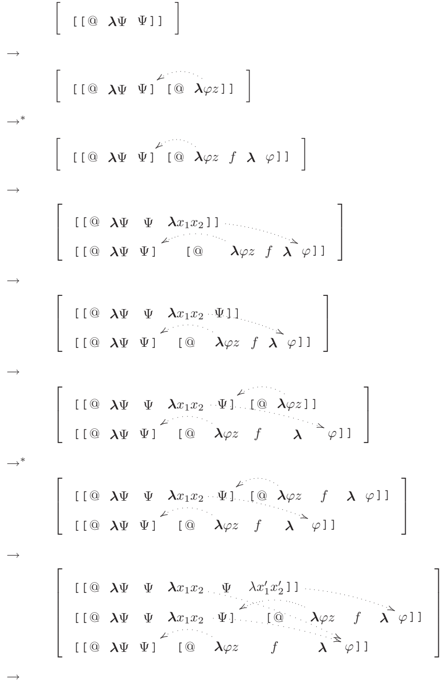
Figure 6: A run of a 3-CPDA (Part 1 of 3).
