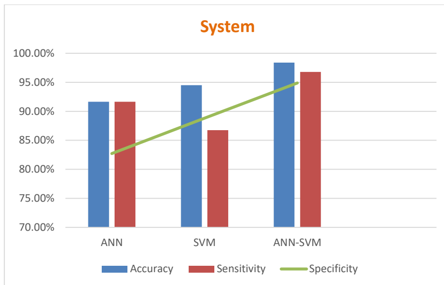
Figure 6: Accuracy of the Hybrid System.
