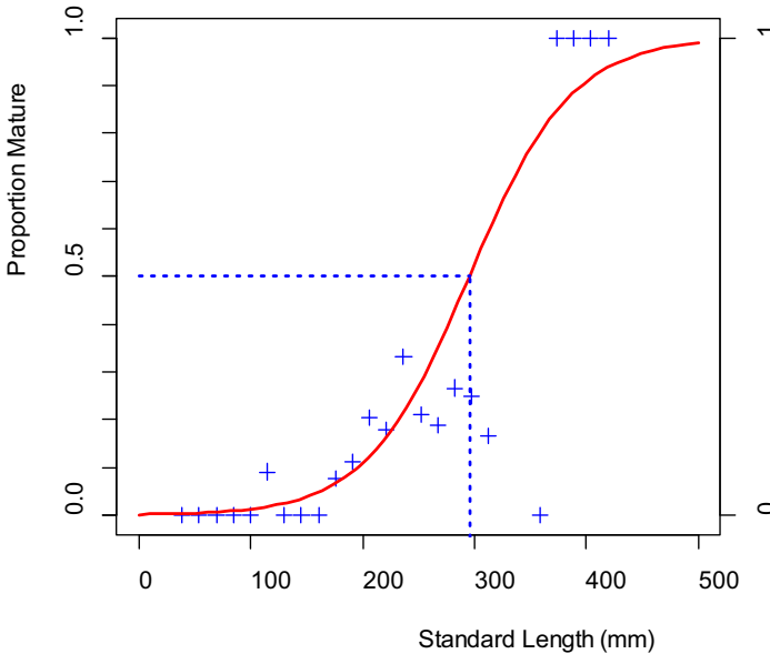
Fig. 3. Fitted logistic regression for proportion of mature Nile tilapia ( O. niloticus ) by standard length with L_{50}=295 mm shown in blue ( N=258 ) in NT2 Reservoir, Lao, PDR. The current mean length of fish at first capture was L_c=210.38 mm.
