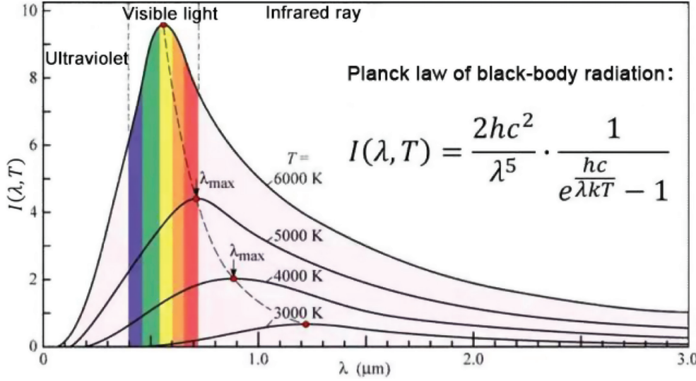
Figure 1. Experimental curves of black-body radiation.
