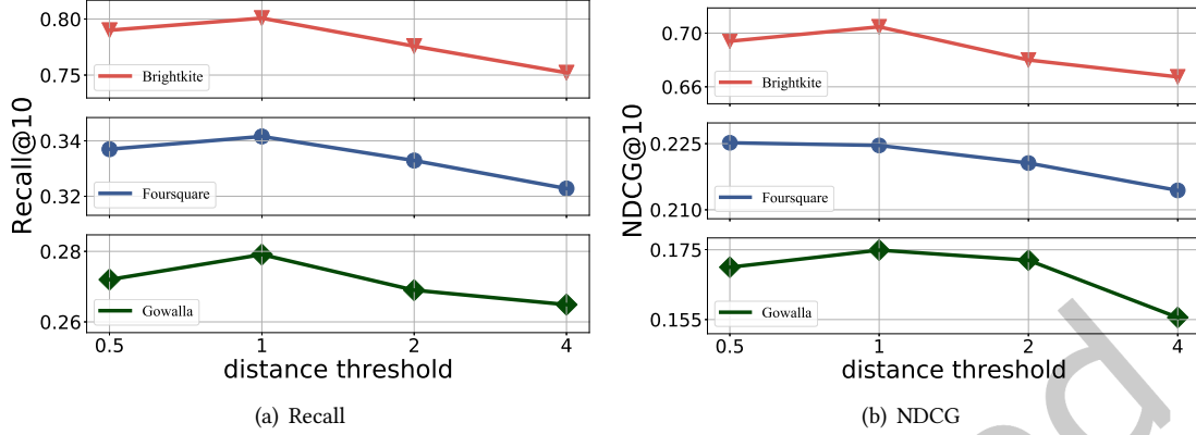
Fig. 9. Effect of distance threshold \Delta d
