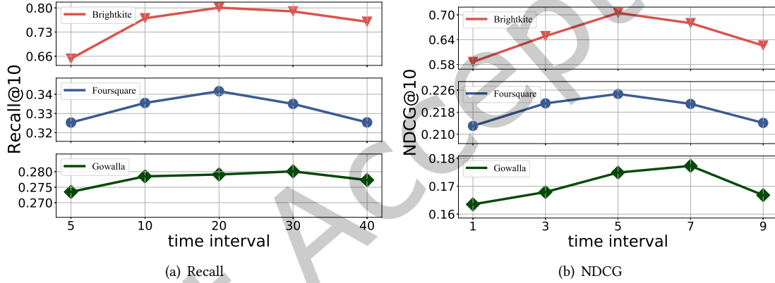
Fig. 10. Effect of time interval \Delta t
