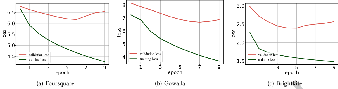
Fig. 6. Loss variations of three datasets
