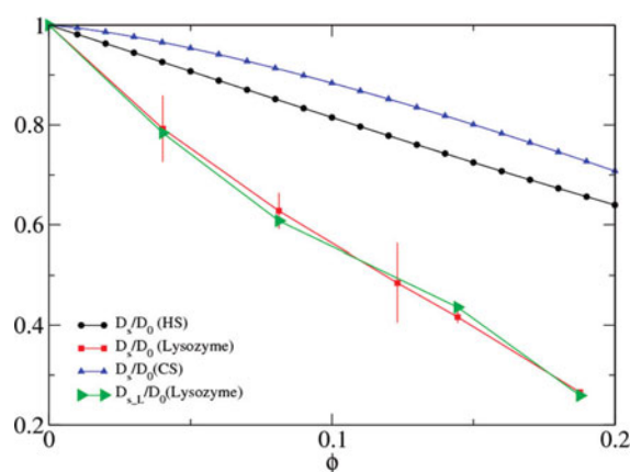
Fig. 19. Comparison of normalized long-time self-diffusion coefficient, D_{s,L}/D_0 and normalized short-time self-diffusion coefficient, D_t/D_0 , as a function of volume fraction. Figure reproduced with permission from Liu et al. (2010). Copyright American Chemical Society.
