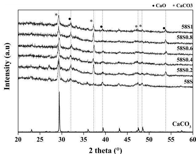
Figure 3: XRD spectra of samples after calcination at 600°C
