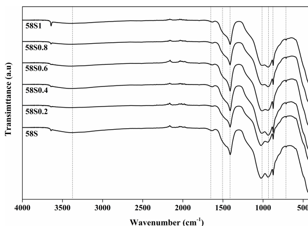
Figure 2: FTIR spectra of samples after heat treatment at 600^\circ\text{C}
