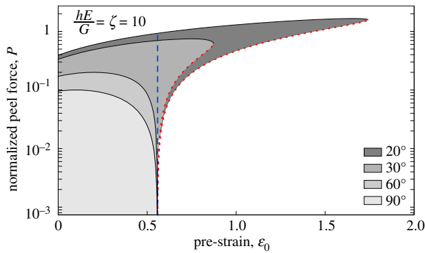
Figure 4. ‘Stability envelopes’ for tape peeling at varying tape pre-strains and peel angles \phi . If the strain exceeds a minimum strain \varepsilon_{\min} (dashed, vertical blue line), stable attachment requires the application of the minimum force to stabilize the contact (dotted red line). In this regime, spontaneous detachment occurs whenever the applied force drops below this lower bound, providing a rapid and efficient detachment mechanism. (Online version in colour.)
