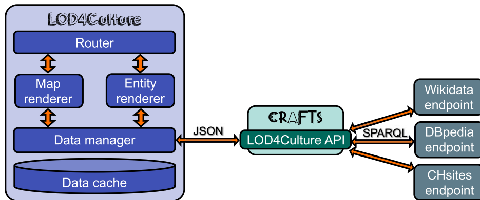
Fig. 1. Architecture of LOD4Culture.
