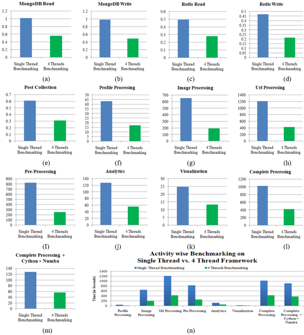
Figure 8. (a) to (m) are displaying the bench-marking on each separate process and (n) is displaying the whole bench-marking in one glance
