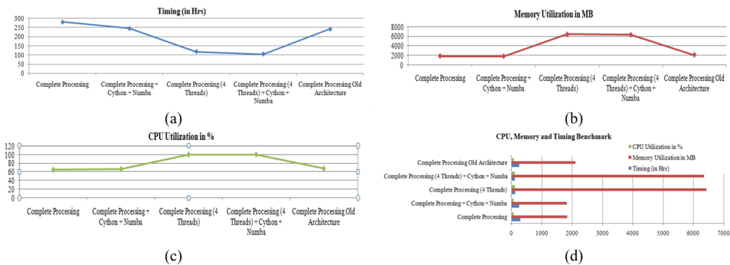
Figure 9. (a) to (c) are displaying the execution timing in Hrs, memory utilization in MB and CPU utilization in percentage and (d) is displaying the whole bench-marking in one glance
