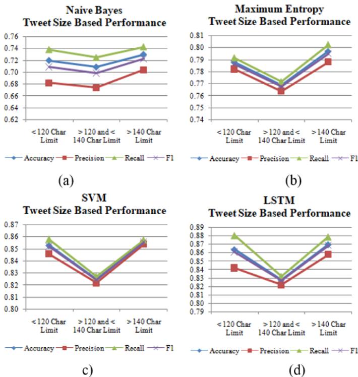
Figure 11. (a) to (d) are displaying the bench-marking on tweet size for Naive Bayes, maximum entropy, SVM, and LSTM respectively
