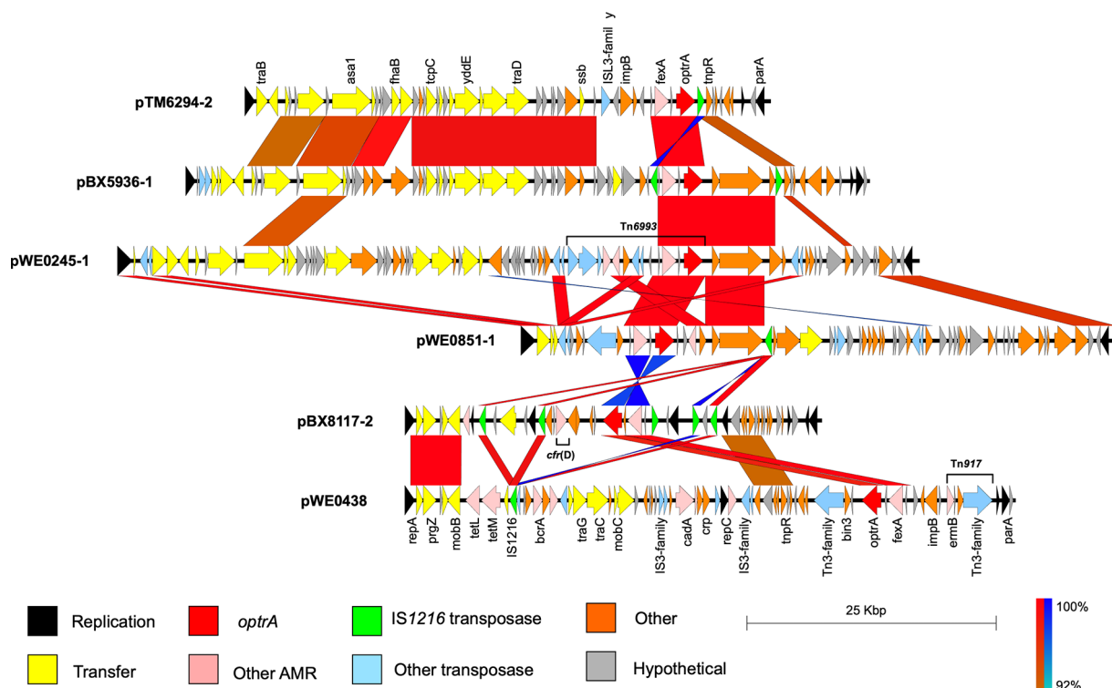
Fig. 1. Alignment of full optrA -positive plasmid sequences. While some sequence similarity is seen between pTM6294-2 and pBX5936-1, in general identity is low between the optrA -positive plasmids, indicating optrA has mobilized to multiple plasmid backbones. Arrows indicate coding sequences, coloured blocks between each sequence indicate regions with BLASTN sequence identity \geq 90\% and length >680 bp. Blue identity blocks indicate inverted sequence.
