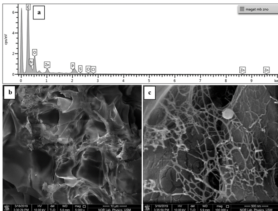
Figure 4. FESEM-EDX micrographs of MAGAT added with methylene blue and ZnO (a) EDX data, and the FESEM micrographs at (b) 5000 \times and (c) 100000 \times .
