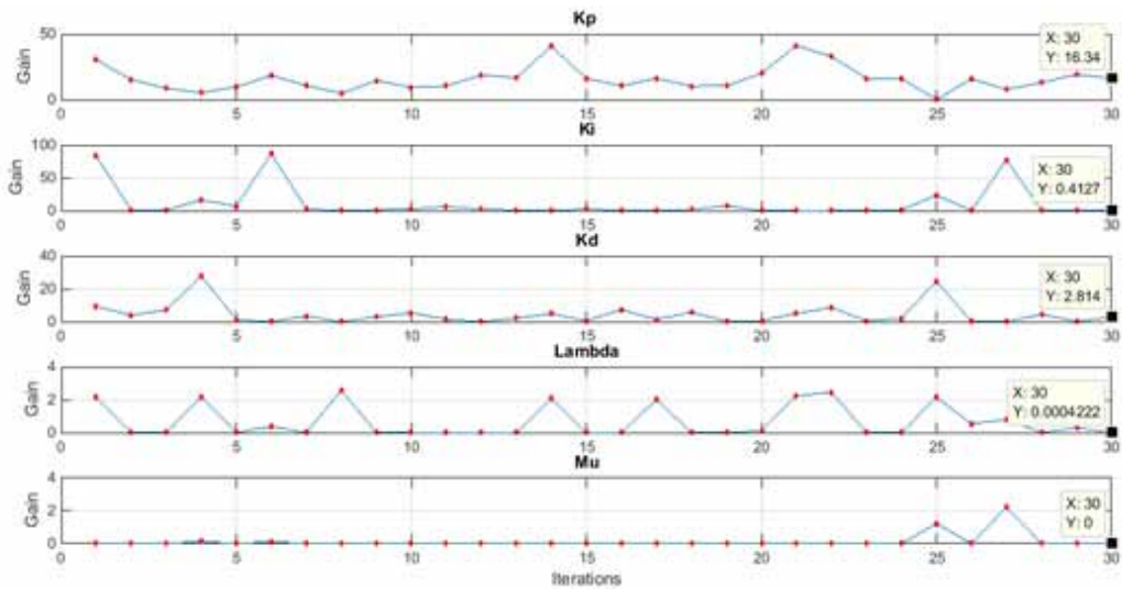
Figure 26. Convergence of the GA-FOPID algorithm through the iterations of I_L
