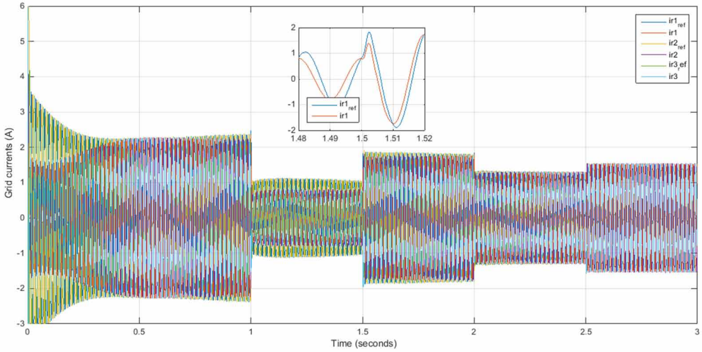
Figure 15. Grid Currents (GA-PID)
