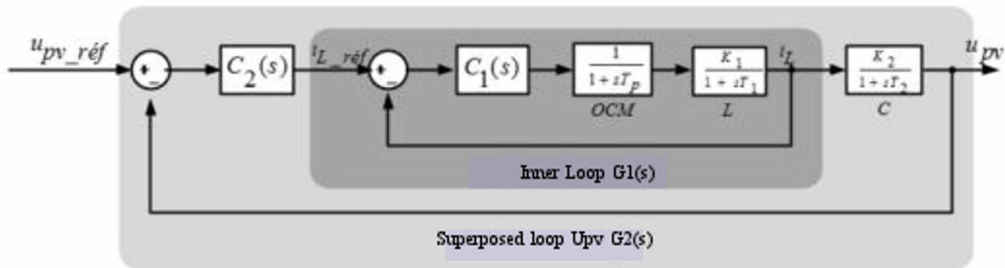
Figure 9. The simplified block diagram of the process
