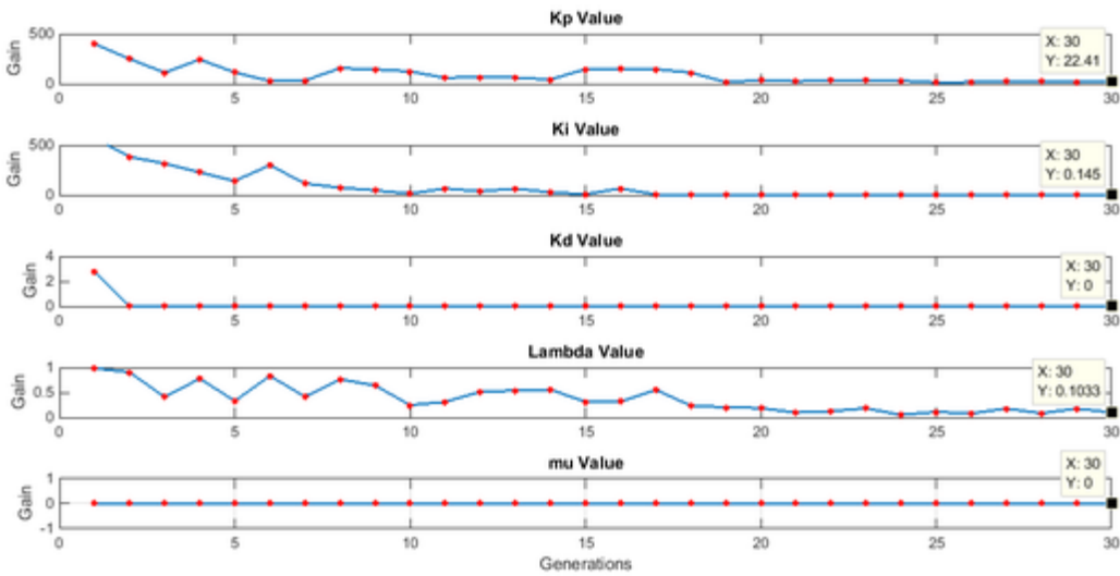
Figure 25. Convergence of the GA-FOPID algorithm through the iterations of U_{pv}
