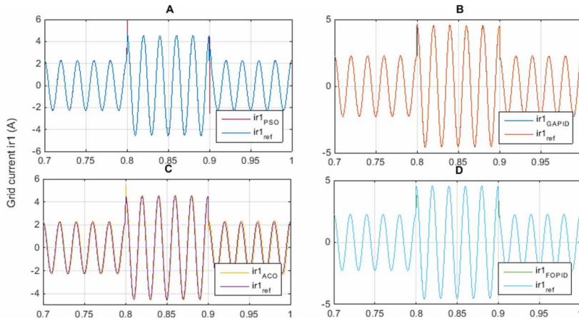
Figure 18. Voltage dip effect on grid currents without limitation by using: A: PSO-PID; B: GA-PID; C: ACO-PID; D: GA-FOPID
