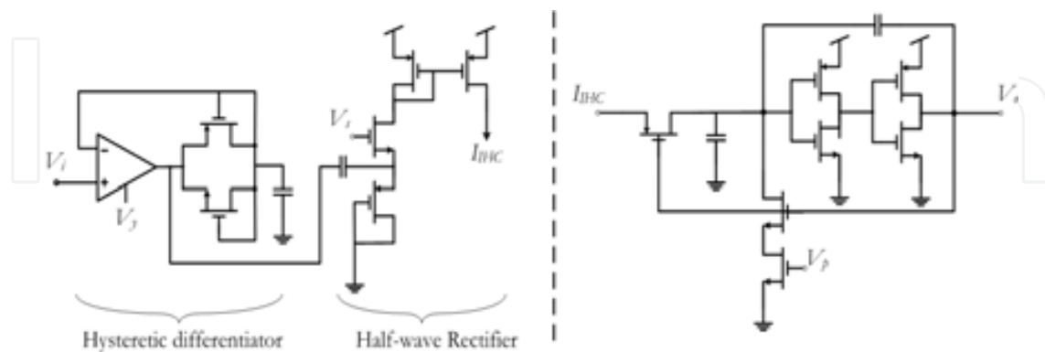
Fig. 6. The IHC (left) and SGN circuit models (right). The input V_i from the BM filtering stage is a time-varying voltage waveform. The hysteretic differentiator, biased with a voltage V_y performs time-differentiation and logarithmic compression. The output from the hysteretic differentiator goes to a half-wave current rectifier circuit. The uni-directional output current from the IHC circuit goes to the SGN circuit which converts it into fixed-width, fixed-height voltage pulses at the output V_o . The bias voltage V_p sets the pulse width with V_o pulsating between the supply and ground; adapted from Lazzaro (Lazzaro and Mead, 1989a).
