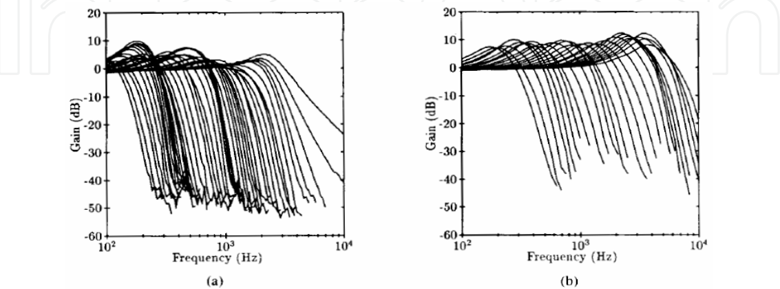
Fig. 11. Frequency response at each voltage tap. (a) Early layout. (b) Improved layout; from Watts (Watts et al., 1992).
