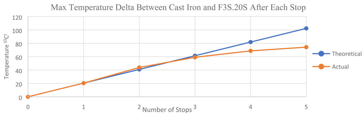
FIG. 5. Comparison between predicted and actual delta between cast iron and F3S.20S (front disc application).
