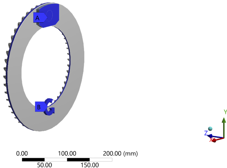
FIG. 16. Illustration of boundary conditions for simulation.
