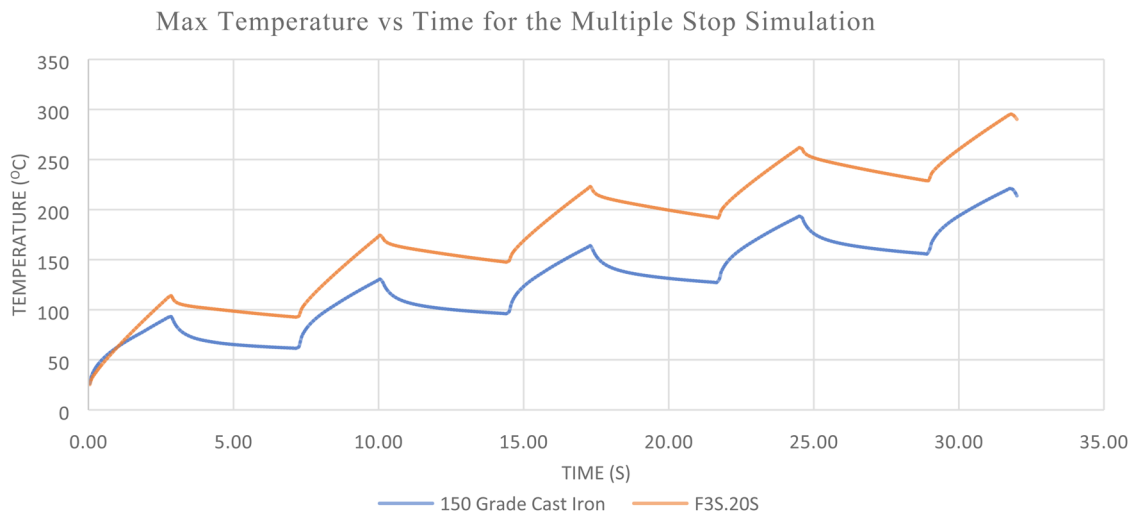
FIG. 4. Results for temperature with multiple stops (front disc application).
