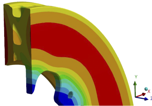
FIG. 7. Simulation results showing single-stop performance of developed disc: (a) front application; (b) rear application.
