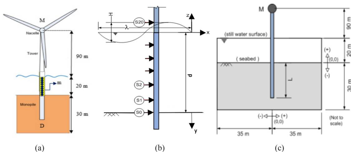
Figure 1. (a) Schematic outlook for the reference OWT [22], (b) wave force application, and (c) numerical modeling of the problem for FE analysis.
