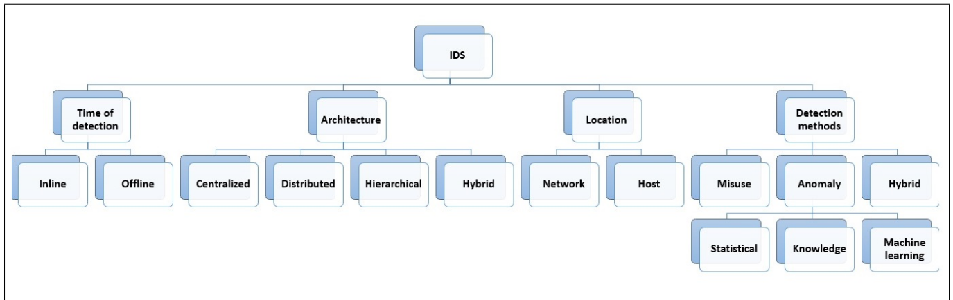
Figure 2. IDS categories
