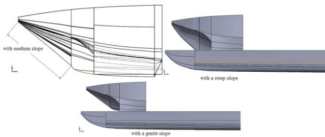
Figure 2. Type of hull designs with different slopes
