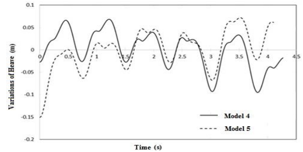
Figure 13. Variation of heave of model 4 and 5 INCAT vessel
