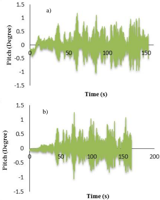
Figure 19. Variations, of pitch a) catamaran b) INCAT at the center of mass in the experimental test ( \zeta=17 cm)
