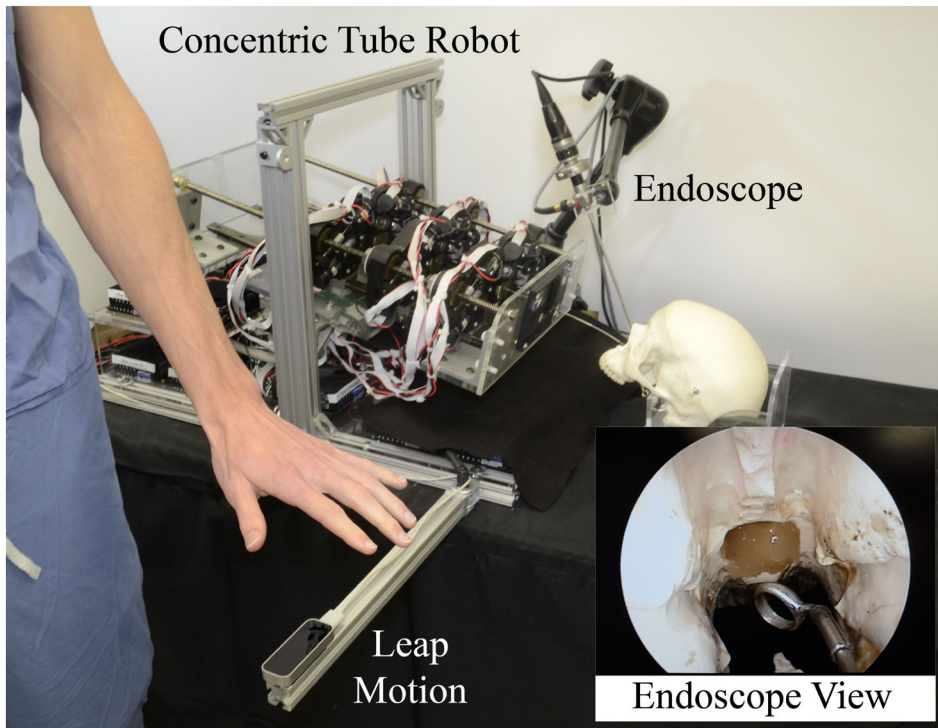
Fig. 4. Experimental setup for phantom tumor resection experiments.
