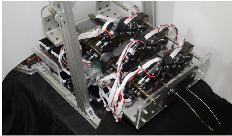
Fig. 2. The actuation unit used to translate and rotate the tubes. Each tube is grasped at its base and may be translated and rotated independently of the others, enabling the concentric tube manipulator to bend and elongate.
