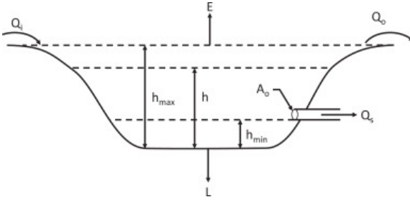
Fig. 1. Schematic diagram of the stormwater basin water balance ( Eq. (1) ): water level depth ( h ), inflow ( Q_i ), overflow ( Q_o ), evaporation ( E ), controlled outflow ( Q_s ) through a structure with area ( A_o ), and exfiltration ( L ). The water level h varies between the invert elevations of the outflow structure ( h_{min} ) and the emergency overflow ( h_{max} ).
