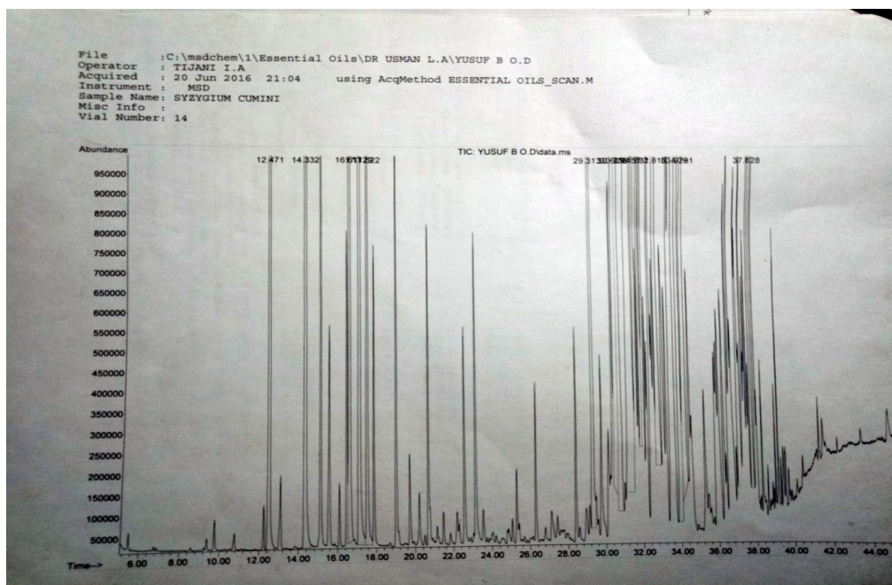
Figure 1: GC-MS Chromatogram Of the essential oil of Syzygium cumini Leaves
