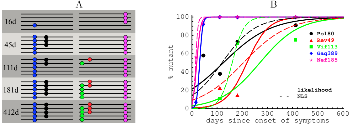
Figure 2: Schematic representation of experimental data on HIV escape from CTL responses (panel A) and fits of the mathematical model to such data (panel B). In panel A, a small number of sequences covering either the 3' or 5' half of the HIV genome has been obtained at 5 different time points. Escape mutations are indicated as colored dots. Typical sequence sample sizes range between 10 and 20. In panel B we show the fits of the mathematical model (eqn. (10)) to experimental data using nonlinear least squares (dashed lines) and likelihood (solid lines) methods. We estimate two parameters: the rate of escape, \varepsilon , and the initial frequency of the escape variant in the population, f_0 . The estimated escape rate obtained by both methods is shown in Table 2.
