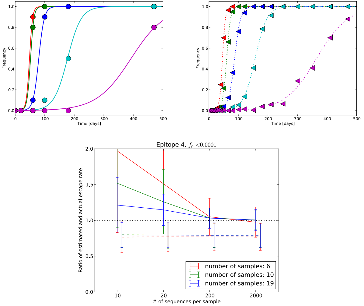
Figure 4: Influence of sampling frequency and sampling depth on escape rate estimate fidelity. The top left and right panel show mutation frequencies in population samples for infrequent shallow sampling ( n = 10 , left), and more frequent deep sampling ( n = 200 , right). Obviously, more frequent and deeper sampling will improve the estimates. This is quantified in the bottom panel. It shows the mean estimate of the escape rate of epitope 4 and its standard deviation as a function of sampling depth for different sampling frequencies. The estimates are shown relative to the true value of the simulated escape rate, hence a systematic deviation from one represents a bias. The dashed lines show the results of fitting only the escape rate, \epsilon , while fixing f_0 . Those fits show a systematic bias towards lower estimates, but have small variance and are insensitive to sample depth or frequency. The solid lines correspond to estimates where both \epsilon and f_0 were fitted, while constraining f_0 to be smaller than 10^{-4} . These fits show much larger variance and a strong bias at small sampling frequencies, but are unbiased at frequent and deep sampling.
