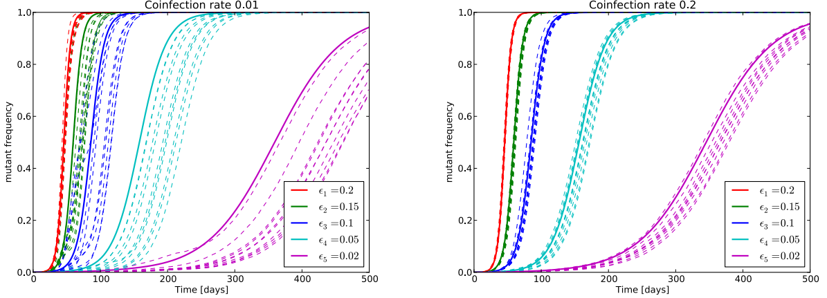
Figure 6: Influence of stochastic effects on CTL escapes. The allele frequency trajectories of the stochastic model (dashed lines, 10 realization) are delayed relative to the deterministic model (solid lines) when coinfection is small (left, coinfection rate is 0.01). This delay is partly due to interference between escapes, as it is strongly reduced at increased coinfection frequency (right, coinfection rate is 0.2). Population size is 10^6 .
