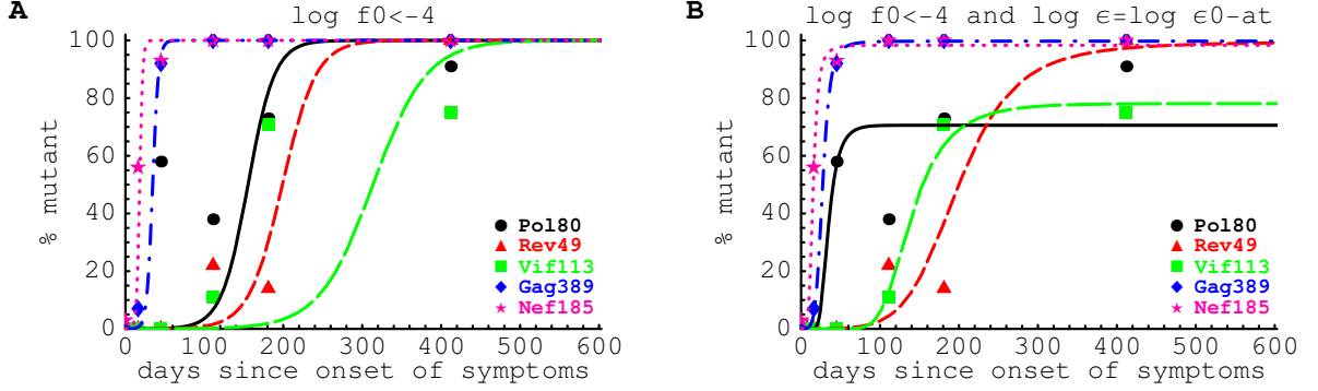
Figure 3: Constraining the initial mutant frequency, f_0 , increases the estimate of the escape rate. By adding an extra penalizing term 10^{10^5(f_0 - f_c)} to the log-likelihood (eqn. (16)) we constrain the initial mutant frequency to not exceed the value f_c = 10^{-4} . The constraint results in much higher estimates of the escape rate (panel A and Table 3). The model that assumes that escape rate changes over the course of infection (panel B and eqn. (13)) improves the fit of the constrained model to data in 3 out of 5 epitopes (Table 3).
