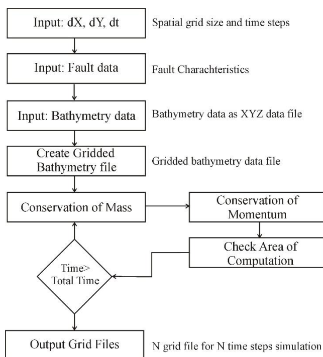
Figure 3. Processing routines of tsunami propagation models used in this paper.
