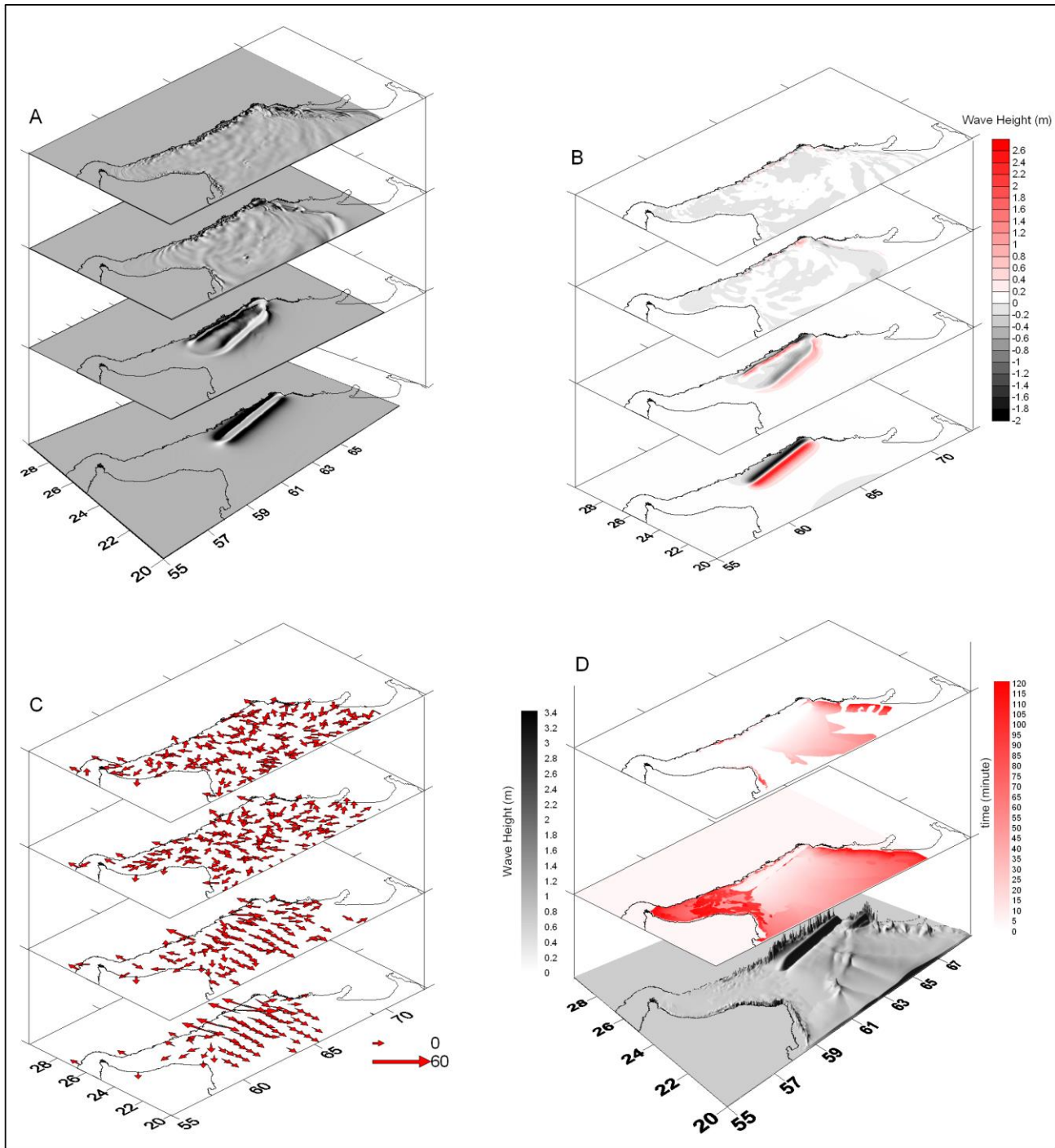
Figure 6. 3D analysis of tsunami propagation model in the Makran region. (a) 3D view of wave propagation at different times. (b) Maximum wave height at different times. (c)- Wave vector of tsunami propagation at different times. Layers in figures A to C from bottom to top show the tsunami wave characteristics at 0 (initial condition), 10, 60 and 120 minutes following tsunami generation. (d) Miscellaneous plots of propagation characteristics: from bottom to top, maximum wave height of tsunami after 120 minutes of modeling; arrival time of maximum wave height; and arrival time of the first 2.5 meter and more wave tsunami.
