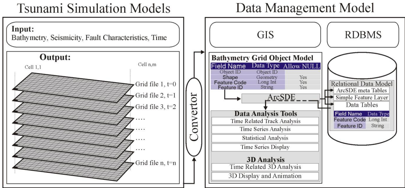
Figure 5. Schematic view of the proposed combined modeling and data management system for tsunami propagation and data analysis.
