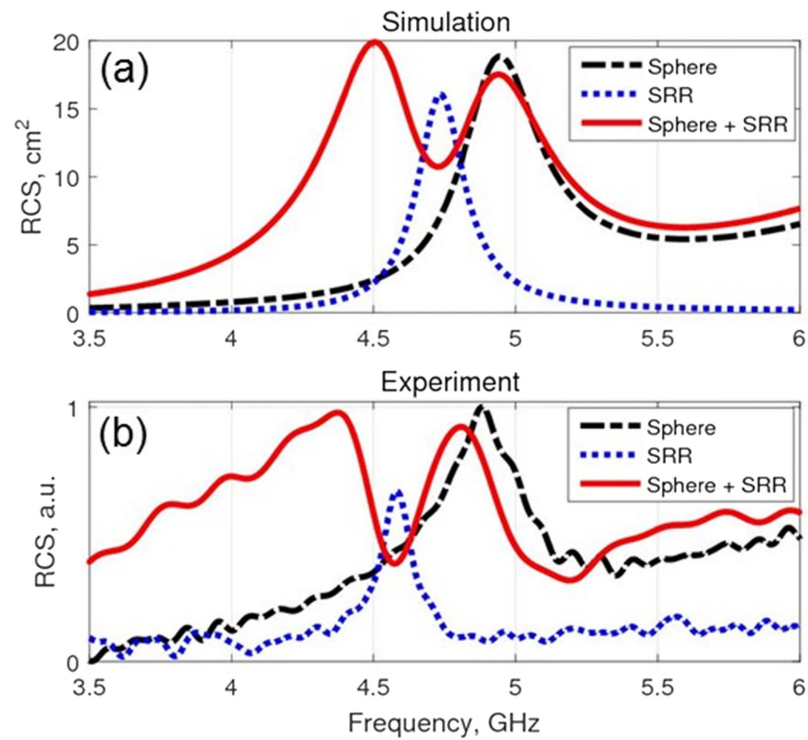
Figure 3. Scattering cross sections of individual meta-atoms and hybrid metamolecule. Individual meta-atoms (SRR and sphere) exhibit strong magnetic dipole resonances shown by dotted (SRR) and dashed (sphere) curves, as observed in (a) numerical simulations and (b) experiment. Being combined into the hybrid metamolecule, the magnetic response demonstrates a splitting of resonances responsible for the formation of the AFM order.
