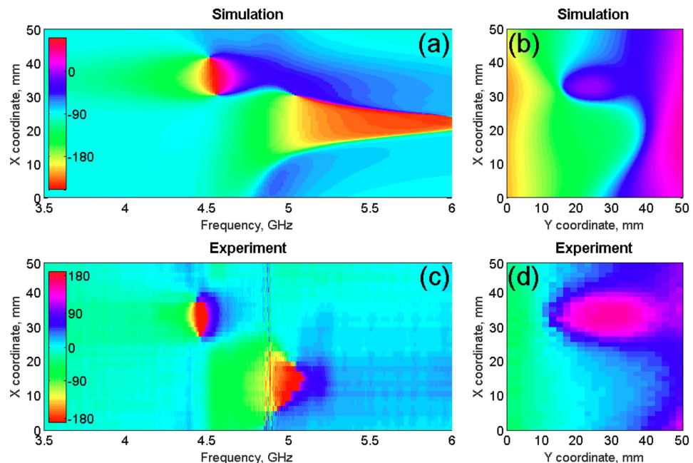
Figure 4. Phase structure of a single hybrid metamolecule. (a), (c) Spectral variation of the magnetic field phase above the hybrid metamolecule along the OX line indicated in figure 2(b), calculated theoretically and measured experimentally. (b), (d) Two-dimensional phase distribution in the plane on top of the hybrid metamolecule at the distance 1 mm above and the resonant frequency 4.73 GHz.
