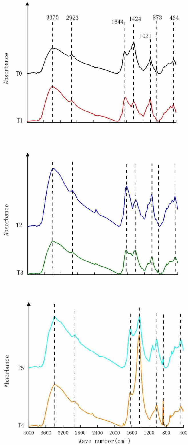
Figure 9. FTIR spectrums of pre-composting and post-composting of treatments
