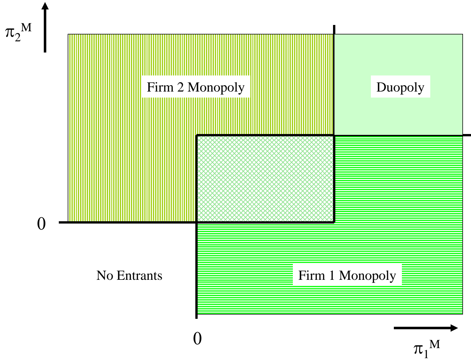
Figure 1. Monopoly and Duopoly Entry Thresholds
