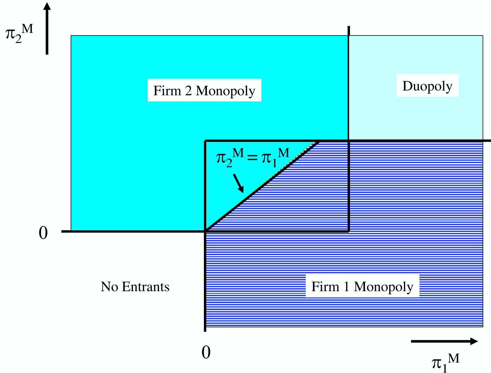
Figure 2. Multi-Stage Sequential Monopoly Model
